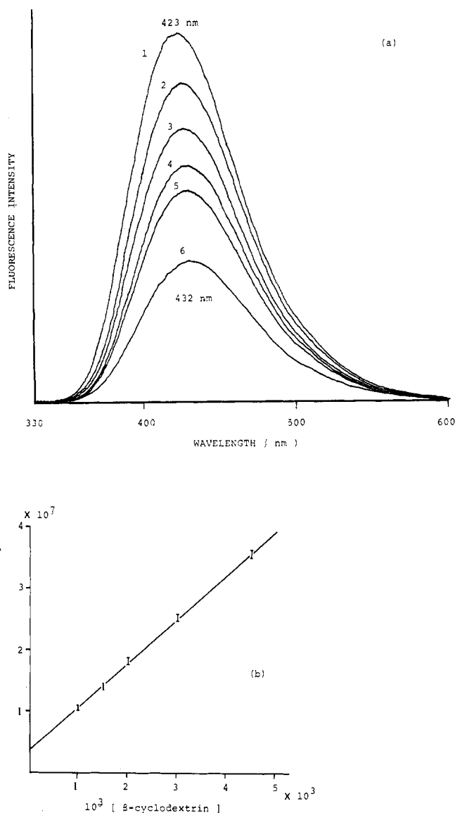
Figure 1. (a) Fluorescence spectrum of 2-methylhydronaphthoquinone-1,4 ( 1 \times 10^{-5} M) in the presence of \beta -cyclodextrin: (1) 10^{-3} M, (2) \frac{2}{3} \times 10^{-3} M, (3) 0.5 \times 10^{-3} M, (4) \frac{1}{3} \times 10^{-3} M, (5) \frac{2}{9} \times 10^{-3} M, and (6) in the absence of \beta -cyclodextrin in phosphate buffer at pH 3.55 (30% methanol by volume). Excitation wavelength 312 nm. (b) Benesi-Hildebrand plot of the fluorescence intensities. K_{\text{ass}} = 490 \text{ M}^{-1} .
