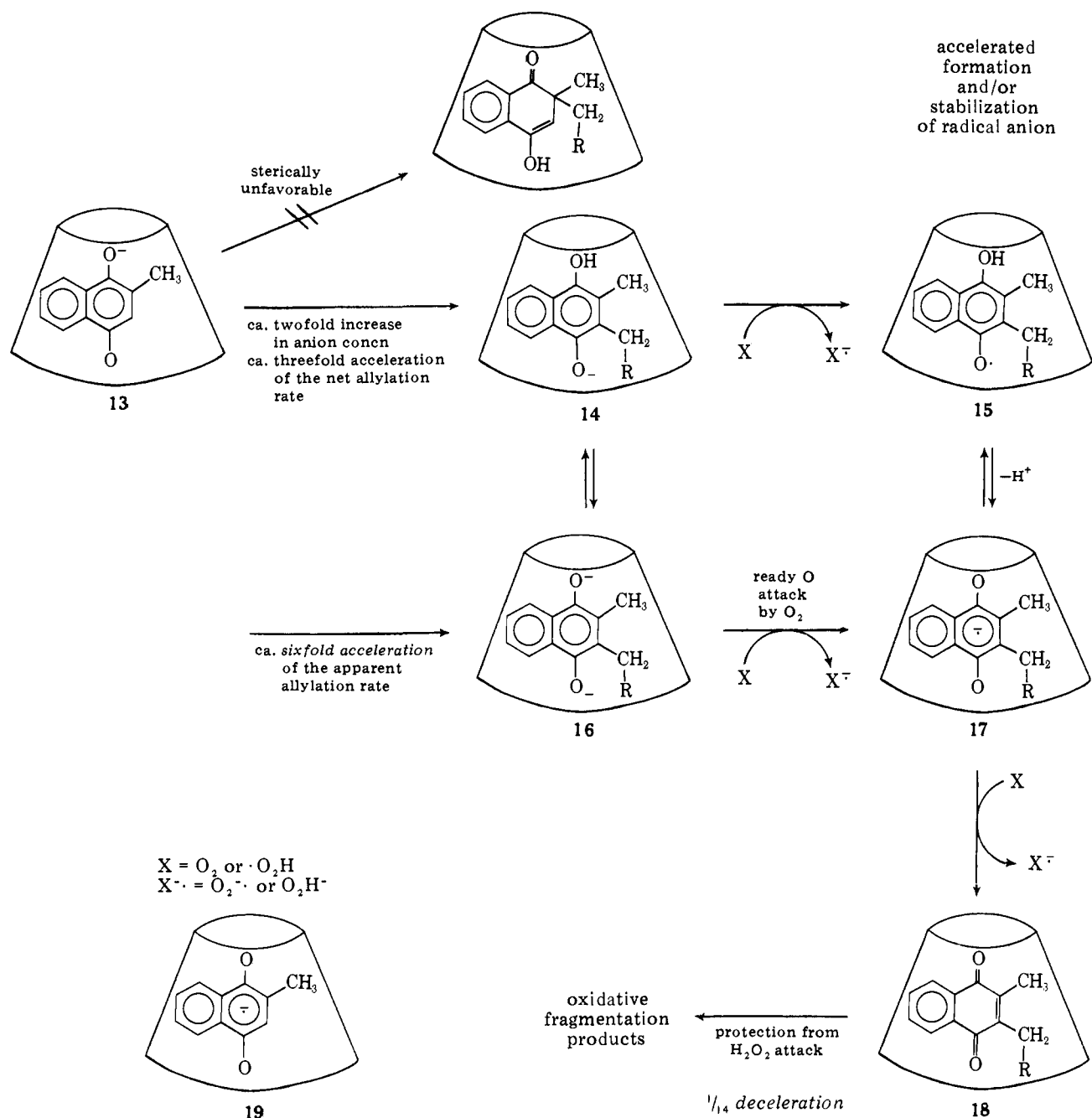
Scheme I. \beta -Cyclodextrin Catalysis
