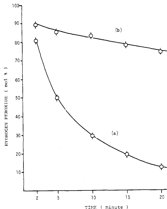
Figure 3. Quantitative determination of hydrogen peroxide produced in the oxidation of 2-methylhydronaphthoquinone (5) (0.005 M) in the absence (a) and presence (b) of \beta -cyclodextrin (0.01 M).
