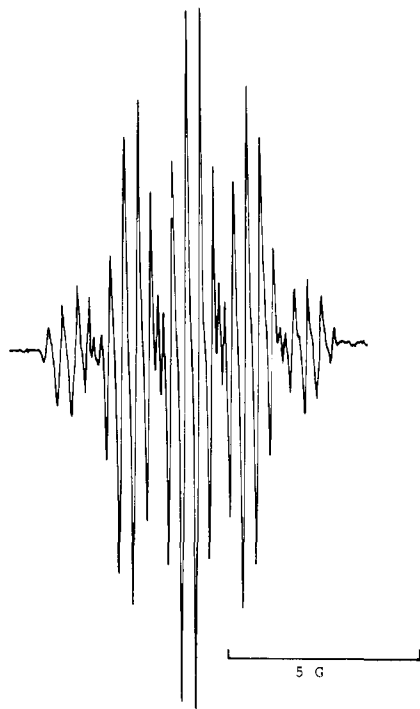
Figure 2. ESR spectrum of 2-methylnaphthoquinone radical anion complexed by \beta -cyclodextrin.
